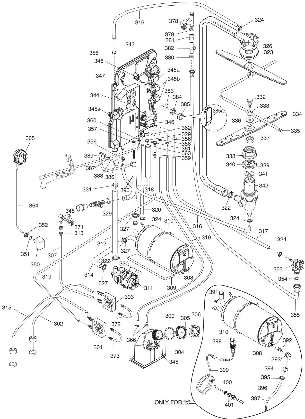
ill. 595665O00_p4B Circuito idraulico / Hydraulic circuit
