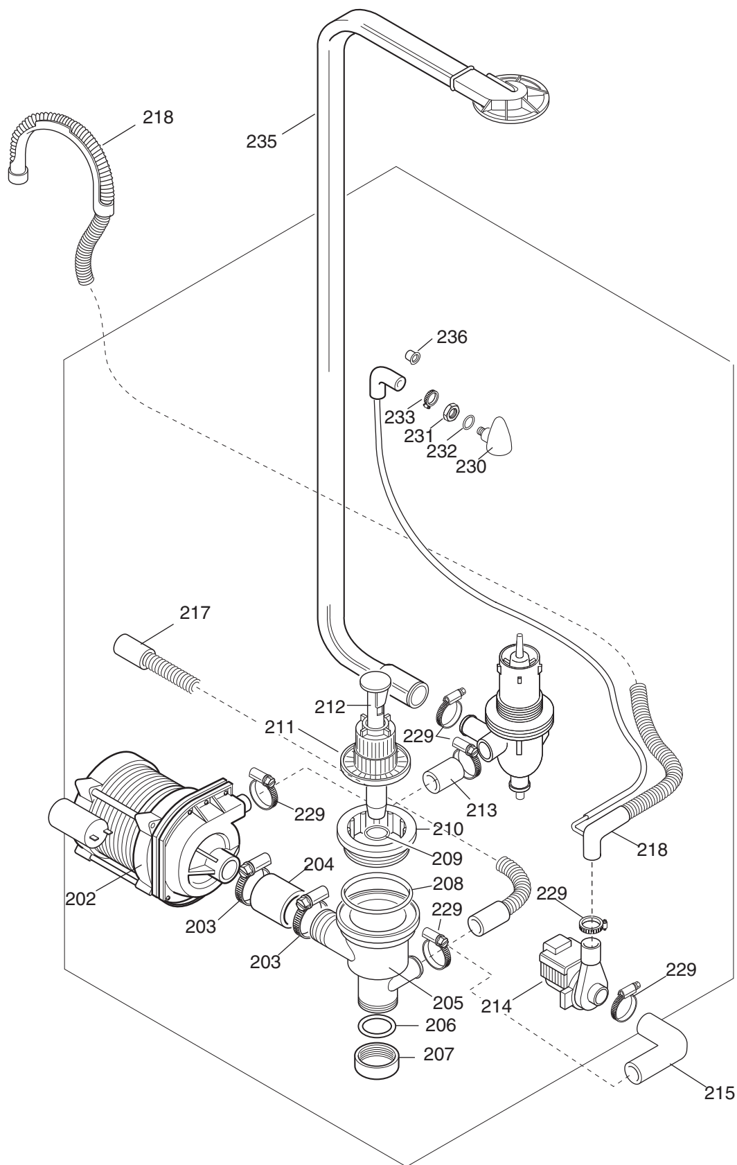
ill. 611002p3 Componenti idraulici / Hydraulic components
